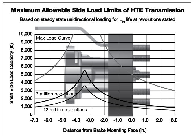
With Brake
